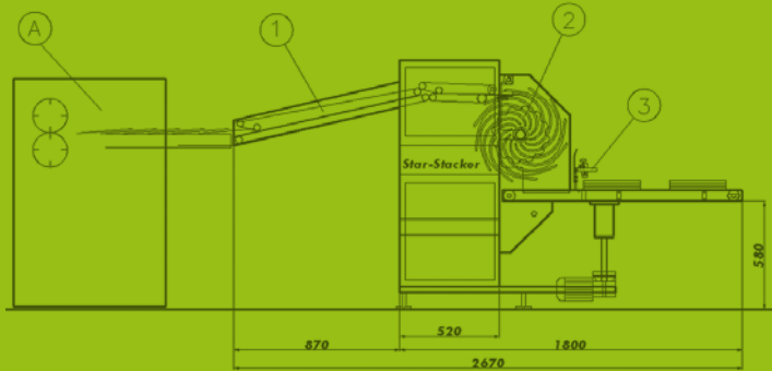
A Sheeter | 1 Infeed belt table | 2 Star wheel | 3 Stacker
